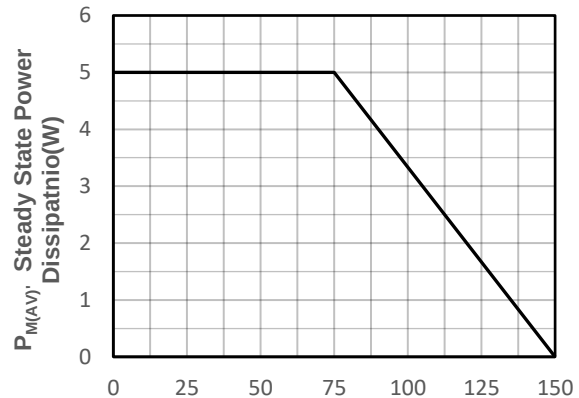
Ambient Temperature T_A ( ^{\circ}\text{C} )
